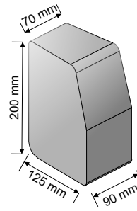
3 Way External Radial
